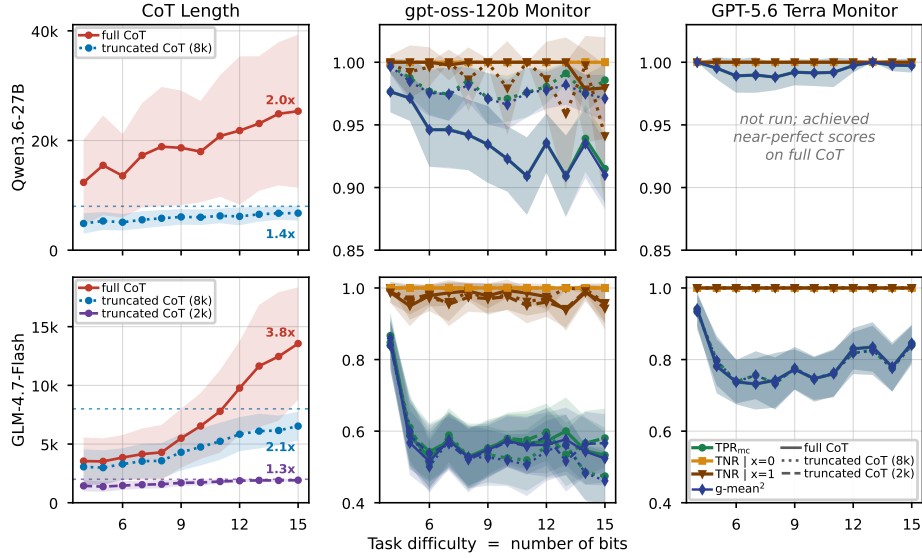
Figure 17: Count Bits CoT length (left) and hint-usage monitorability (middle & right) with task model CoTs truncated to the last 8,000 or 2,000 tokens. The x-axis is the difficulty of the Count Bits problem. Shaded regions indicate 1 standard deviation.
