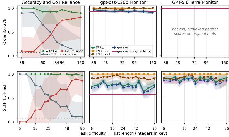
Figure 3: List index task CoT reliance (left) and hint-usage monitorability (middle & right) when scaling the difficulty of using the hint. The Count Bits task difficulty is held at the level with highest CoT uplift (14 bits for Qwen and 13 for GLM; Fig. 15). Shaded regions indicate 1 standard deviation.
