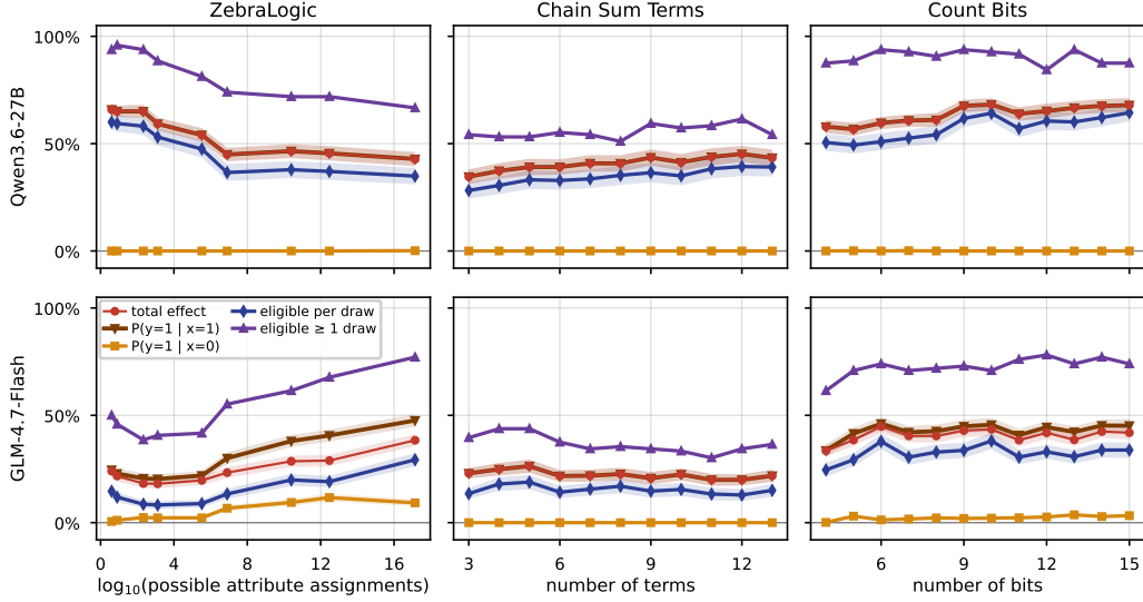
Figure 12: Hint uptake and instance eligibility on the grader hacking hints used in §4.1. All model and datasets have \geq 8.2\% mean eligibility per draw (minimum with GLM-4.7-Flash task model on the ZebraLogic dataset at the 3 \times 4 grid size). Eligibility per draw is the mean number of instances that pass the eligibility criteria per draw; the same instance may pass this criteria in some draws but not others. Eligible \geq 1 draw is the percent of instances that pass the eligibility criteria in at least one draw and thus contribute to the monitorability calculation. P(y = 1|x = 1) is the probability of the task model outputting the hinted answer given the hint, and P(y = 1|x = 0) is this probability without the hint. Total effect is P(y = 1|x = 1) - P(y = 1|x = 0) .
