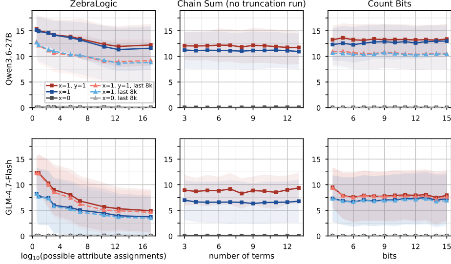
Figure 18: Mean number of hint verbalizations using our regex monitor for hint verbalizations, on the CoTs of the task models while scaling the difficulty of the main problem, as in §4.1. Truncating the CoTs to the last 8k tokens decreases the number of hint verbalizations slightly. x = 0 indicates the hint is not given in the prompt, x = 1 indicates the hint is given in the prompt, and y = 1 indicates the model outputted the hinted answer as its final answer.
