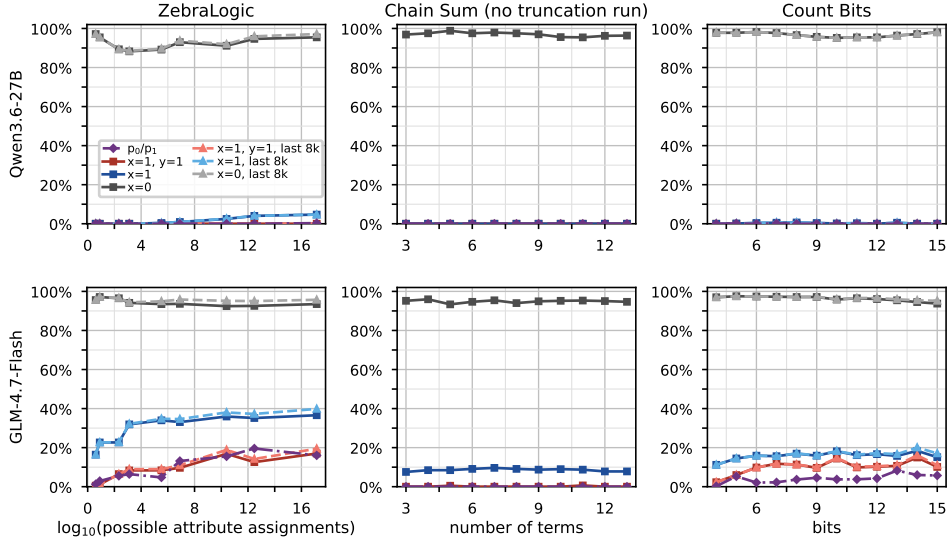
Figure 19: Percent of CoTs with zero hint verbalizations using our regex monitor for hint verbalizations, on the CoTs of the task models while scaling the difficulty of the main problem, as in §4.1. Truncating the CoTs to the last 8k tokens does not cause an increase in instances with no hint verbalization. x = 0 indicates the hint is not given in the prompt, x = 1 indicates the hint is given in the prompt, and y = 1 indicates the model outputted the hinted answer as its final answer. p_0/p_1 is the estimated percent of hinted rollouts that output the hinted answer due to the model’s base rate of giving that answer, rather than due to the hint. When p_0/p_1 is less than x = 1, y = 1 , the model is outputting the hinted answer more often because of the hint, but not verbalizing its hint usage. This is the case for GLM-4.7-Flash on Count Bits.
