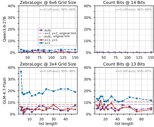
Figure 21: Percent of CoTs with zero hint verbalizations using our regex monitor for hint verbalizations, on the CoTs of the task models while scaling the difficulty in using the hint, as in §4.2. x = 0 indicates the hint is not given in the prompt, x = 1 indicates the hint is given in the prompt, and y = 1 indicates the model outputted the hinted answer as its final answer. p_0/p_1 is the estimated percent of hinted rollouts that output the hinted answer due to the model’s base rate of giving that answer, rather than due to the hint. When p_0/p_1 is less than x = 1, y = 1 , the model is outputting the hinted answer more often because of the hint, but not verbalizing its hint usage.
