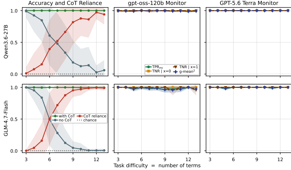
Figure 16: Chain Sum Terms hint-usage monitorability when scaling the difficulty of the unhinted Chain Sum Terms problem. Shaded regions indicate 1 standard deviation. Monitorability is saturated for both task models and monitor models on this dataset, and is not affected by task difficulty or CoT reliance. This is a “success case” of the dataset, though we believe it’s the least representative of real-world monitoring which often covers much longer CoTs.
