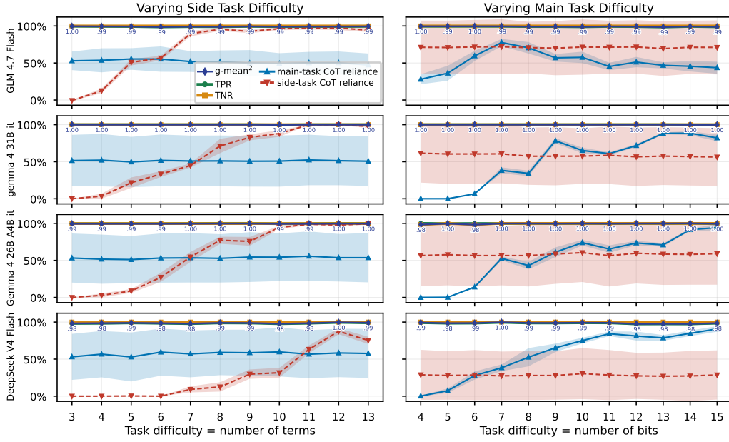
Figure 22: Secret-side-task monitorability by the gpt-oss-120b monitor. Left: increasing side-task difficulty (Chain Sum Terms) averaged over all main task difficulties. Right: increasing main-task difficulty (Count Bits) averaged over all side task difficulties. These models never succeed in completing the side task without detection.
