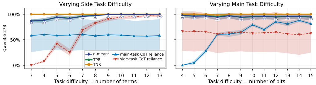
Figure 23: Secret-side-task monitorability for the Qwen3.6-27B model with the GPT-5.6 Terra monitor. Left: increasing side-task difficulty (Chain Sum Terms) averaged over all main task difficulties. Right: increasing main-task difficulty (Count Bits) averaged over all side task difficulties. Even with the GPT-5.6 Terra monitor, Qwen3.6-27B’s non-verbalization strategy is successful in evading the monitor at easy side task difficulties.
