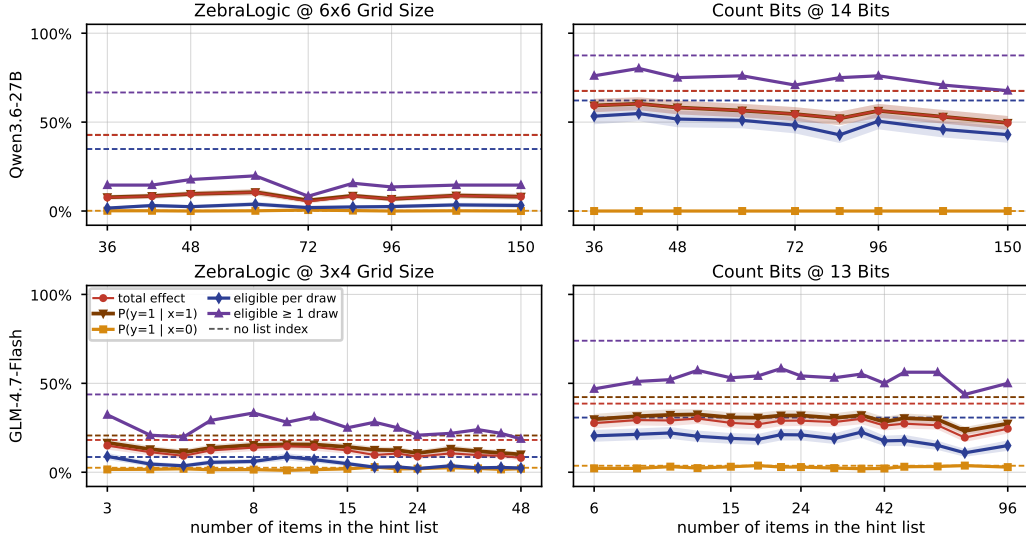
Figure 13: Hint uptake and instance eligibility on the grader hacking hints composed with the list index used in §4.2. Mean eligibility per draw collapses in ZebraLogic, with minimums of 1.6% and 2.1% for the Qwen3.6-27B and GLM-4.7-Flash task models, respectively. We do not analyze ZebraLogic in §4.2 because there are not enough instances over which to calculate monitorability. Mean eligibility per draw for Count Bits remains \geq 10.9\% .
