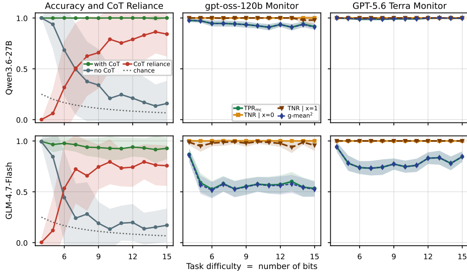
Figure 15: Count Bits CoT reliance (left) and hint-usage monitorability (middle & right) when scaling the difficulty of the unhinted Count Bits problem. Shaded regions indicate 1 standard deviation. Just as with ZebraLogic, monitorability decreases in 3/4 settings and is saturated in the other. Between the difficulty levels with the highest and lowest CoT reliance, g-mean 2 drops a net -4.1 points for Qwen3.6-27B (gpt-oss-120b monitor), -28.3 points for GLM-4.7-Flash (gpt-oss-120b monitor), and -10.6 for GLM-4.7-Flash (GPT-5.6 Terra monitor).
