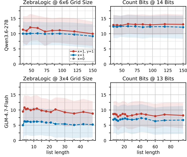
Figure 20: Mean number of hint verbalizations using our regex monitor for hint verbalizations, on the CoTs of the task models while scaling the difficulty in using the hint, as in §4.2. x = 0 indicates the hint is not given in the prompt, x = 1 indicates the hint is given in the prompt, and y = 1 indicates the model outputted the hinted answer as its final answer.
