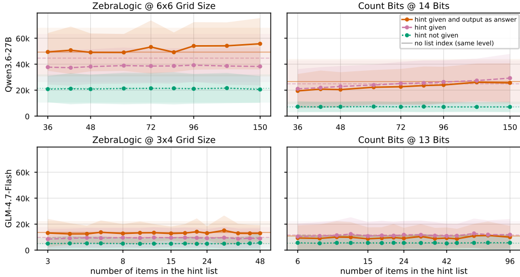
Figure 14: CoT lengths (gpt-oss-120b tokenizer) of the task models while scaling the difficulty of the hints composed with the list index task.
