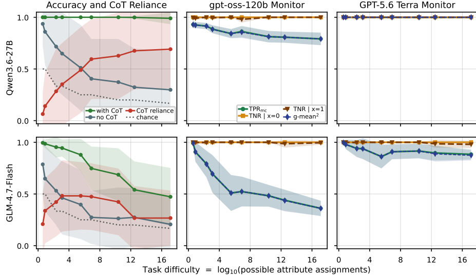
Figure 2: ZebraLogic CoT reliance (left) and hint-usage monitorability (middle & right) when scaling the difficulty of the unhinted ZebraLogic problem. Shaded regions indicate 1 standard deviation. Monitorability decreases with increasing CoT reliance in 3/4 settings: net -13.8 percentage points for Qwen3.6-27B (gpt-oss-120b monitor), -29.7 for GLM-4.7-Flash (gpt-oss-120b monitor), and -5.9 for GLM-4.7-Flash (GPT-5.6 Terra monitor). Qwen3.6-27B (GPT-5.6 Terra monitor) is the exception, retaining perfect scores.
