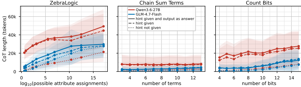
Figure 4: CoT lengths (gpt-oss-120b tokenizer) of the task models as a function of task difficulty.
