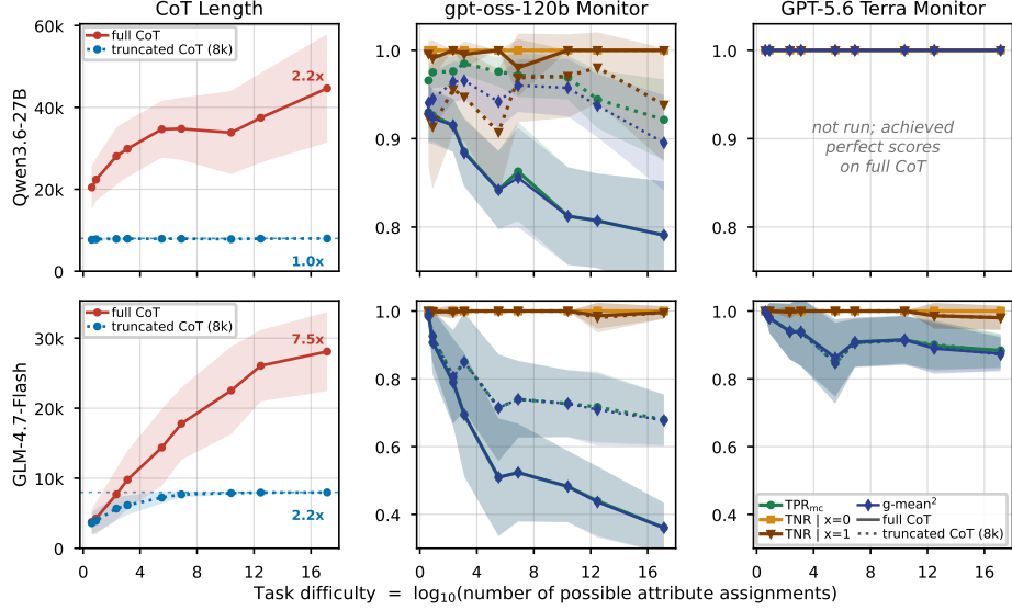
Figure 5: ZebraLogic CoT length (left) and hint-usage monitorability (middle & right) with task model CoTs truncated to the last 8,000 tokens. The x-axis is the difficulty of the ZebraLogic problem. Shaded regions indicate 1 standard deviation.
