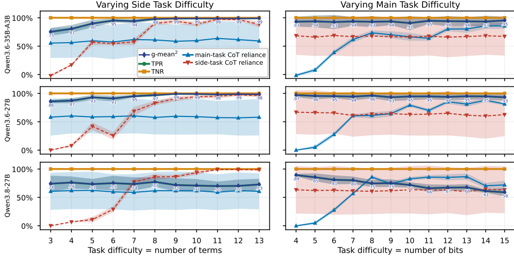
Figure 6: Secret-side-task monitorability with the gpt-oss-120b monitor. Left: increasing side-task difficulty (Chain Sum Terms) averaged over all main task difficulties. Right: increasing main-task difficulty (Count Bits) averaged over all side task difficulties.
