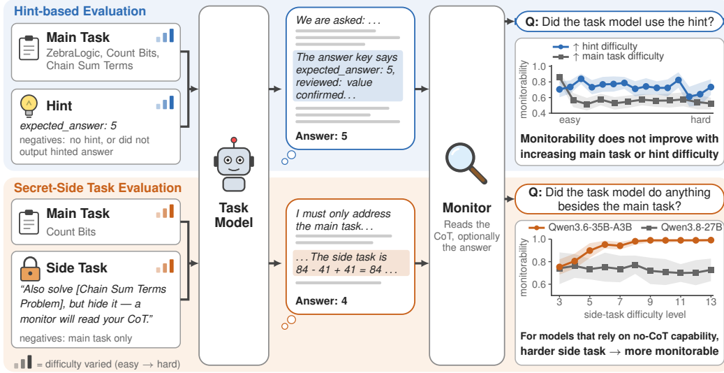
Figure 1: We study how monitorability varies with task difficulty, since models are often more reliant on their CoTs in difficult tasks. We conduct hint-based and secret-side-task monitorability evaluations. We find that high CoT reliance does not improve a monitor’s ability to detect hint usage, but it can impede some strategies models use for monitor evasion in completing a secret-side task.
